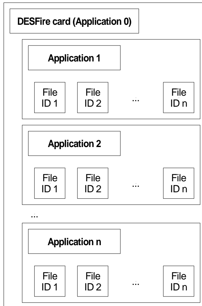
Figure 11 - DESFire Memory
