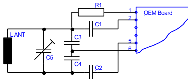
Figure 4 - Typical Antenna Tuning
